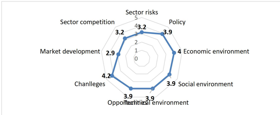
Figure 28: Score of the overall environment by government venture philanthropists
